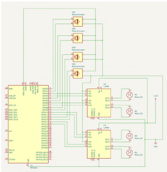
Figure 11: Wiring diagram in KiCAD
