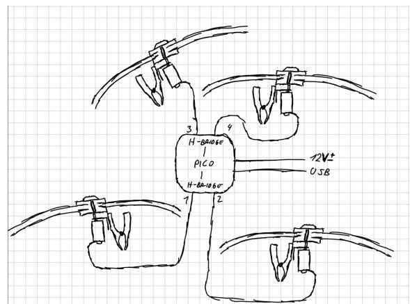
Figure 7: Larger module capable of independently interfacing with DAW
