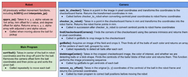
Fig. 9. Class and method structure used for organizing code to complete the lab exercise
