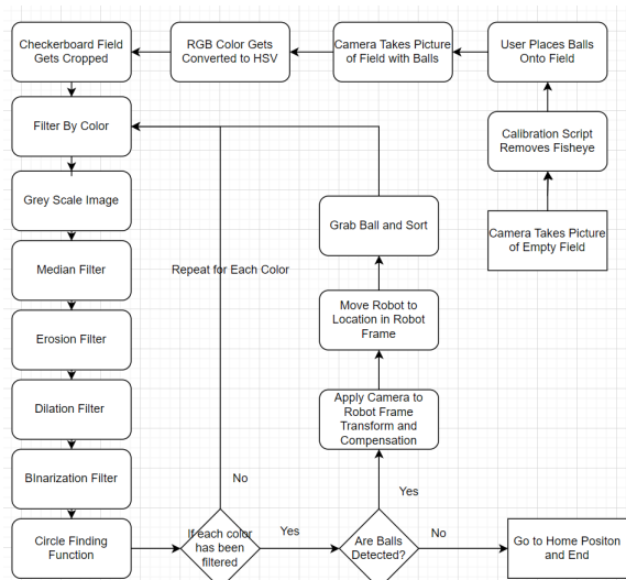
Fig. 8. Flowchart of the entire sorting process completed by the camera and robot
